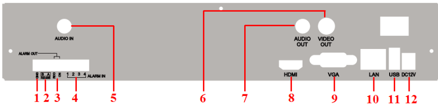
Fig 2-3 Rear Panel for 4-ch
