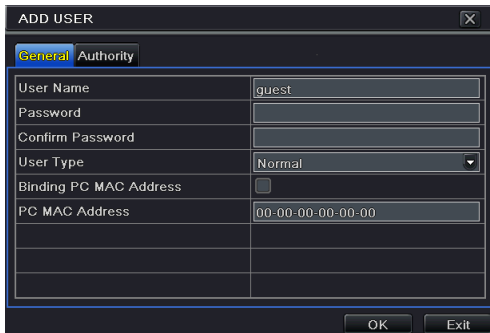
Fig 5-28 Add-General
