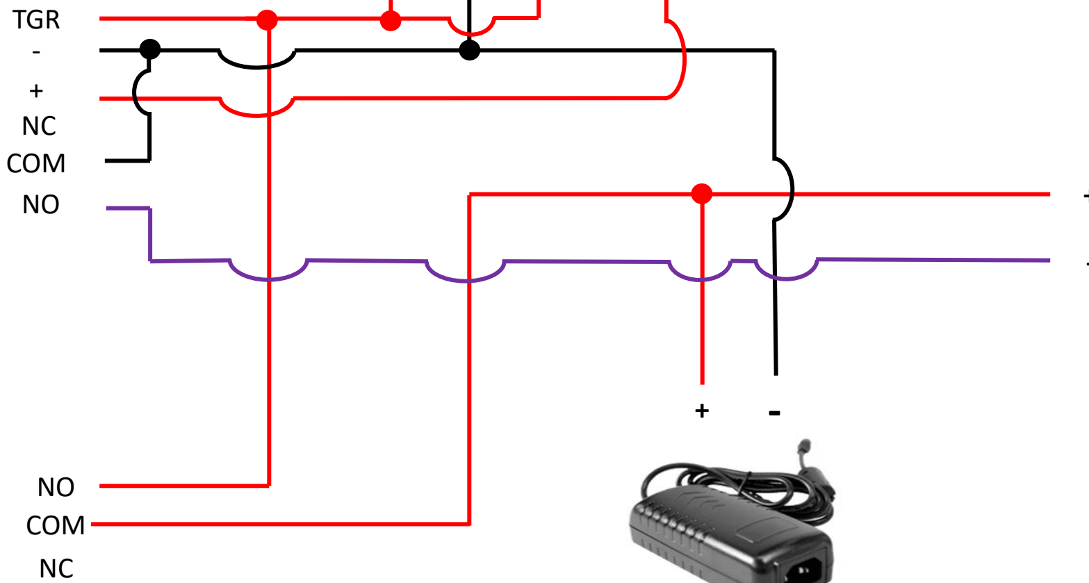
12V | GND | COM | NC | NO
